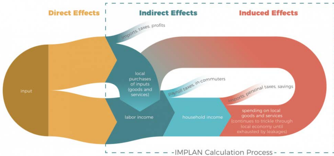
Figure 18: IMPLAN Model 33
